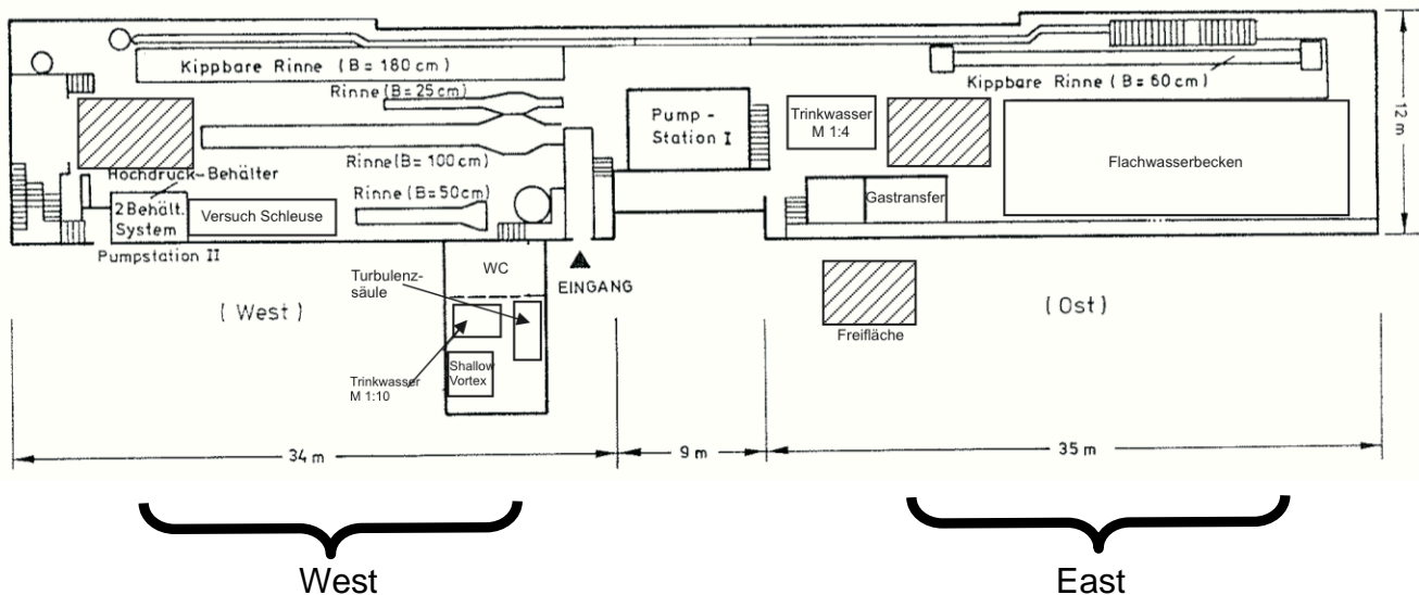
Fig. 2: Water Research Laboratory, 2014
