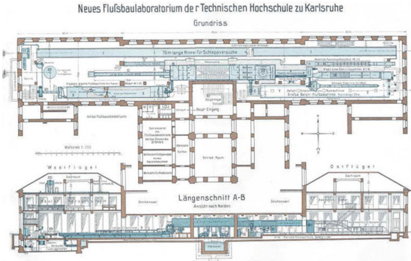
Fig. 1: Water Research Laboratory, 1921
